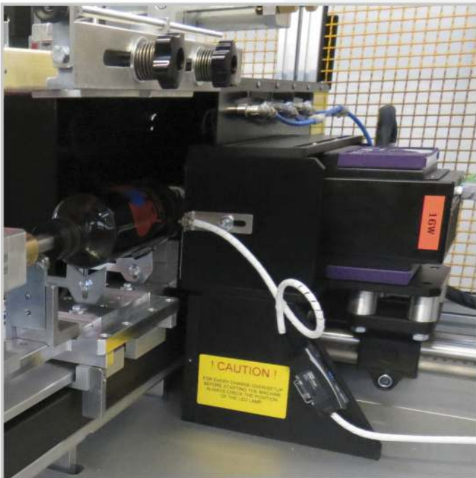
FORNO LED LED DRYER
